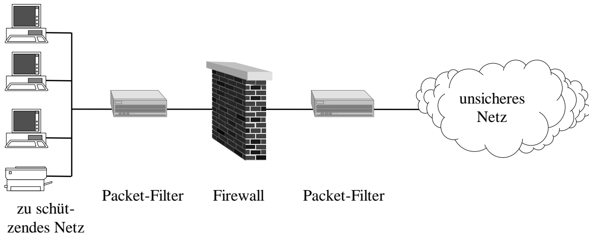
Abbildung 3.4: Screened Gateway (Sandwich-System)
